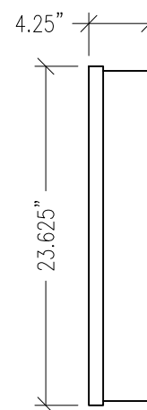
SIDE
