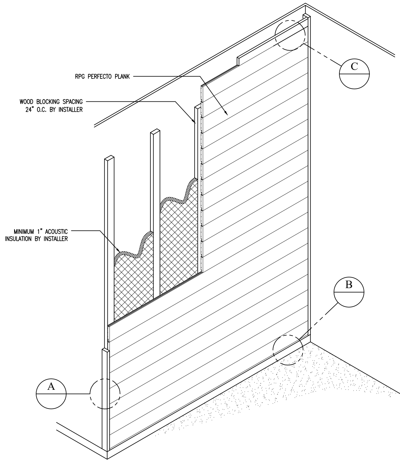
ISOMETRIC VIEW (NTS)
