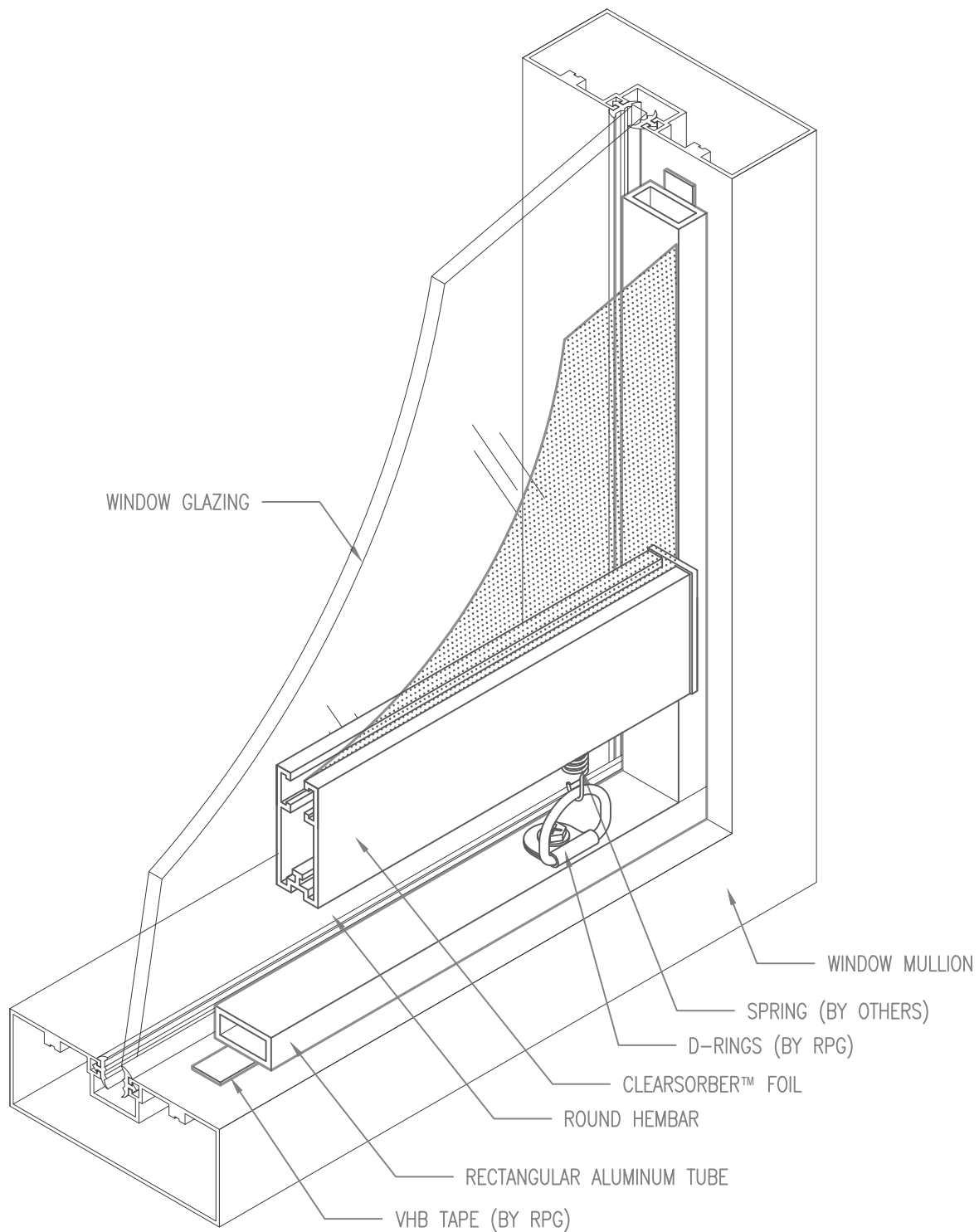
CLEARSORB™ FOIL (SINGLE LAYER) PENETRATION FREE MOUNTING TUBE/D-RING/SPRING/SINGLE HEMBAR MOUNTING
