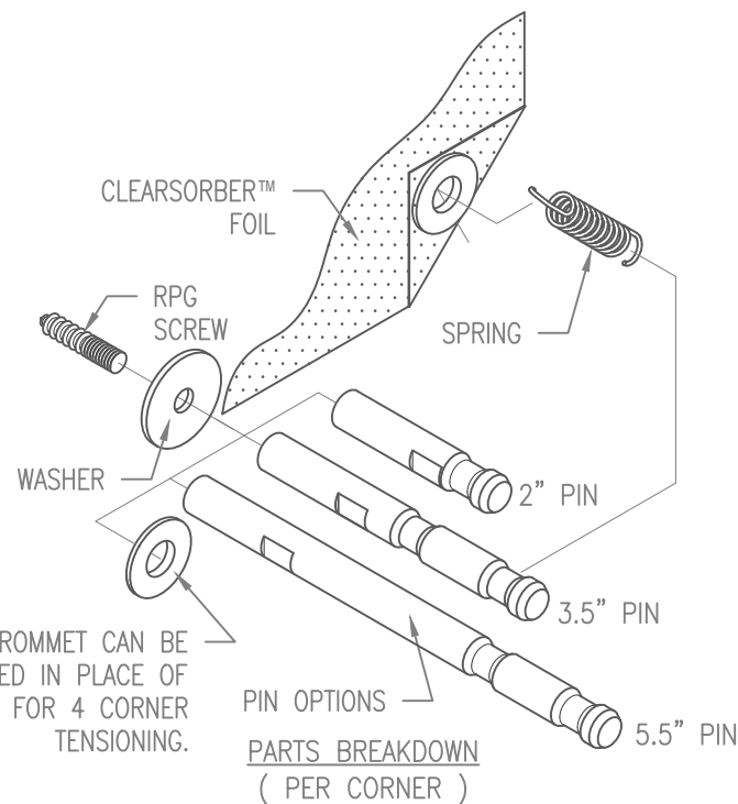
THREE CORNER PIN ATTACHMENT
