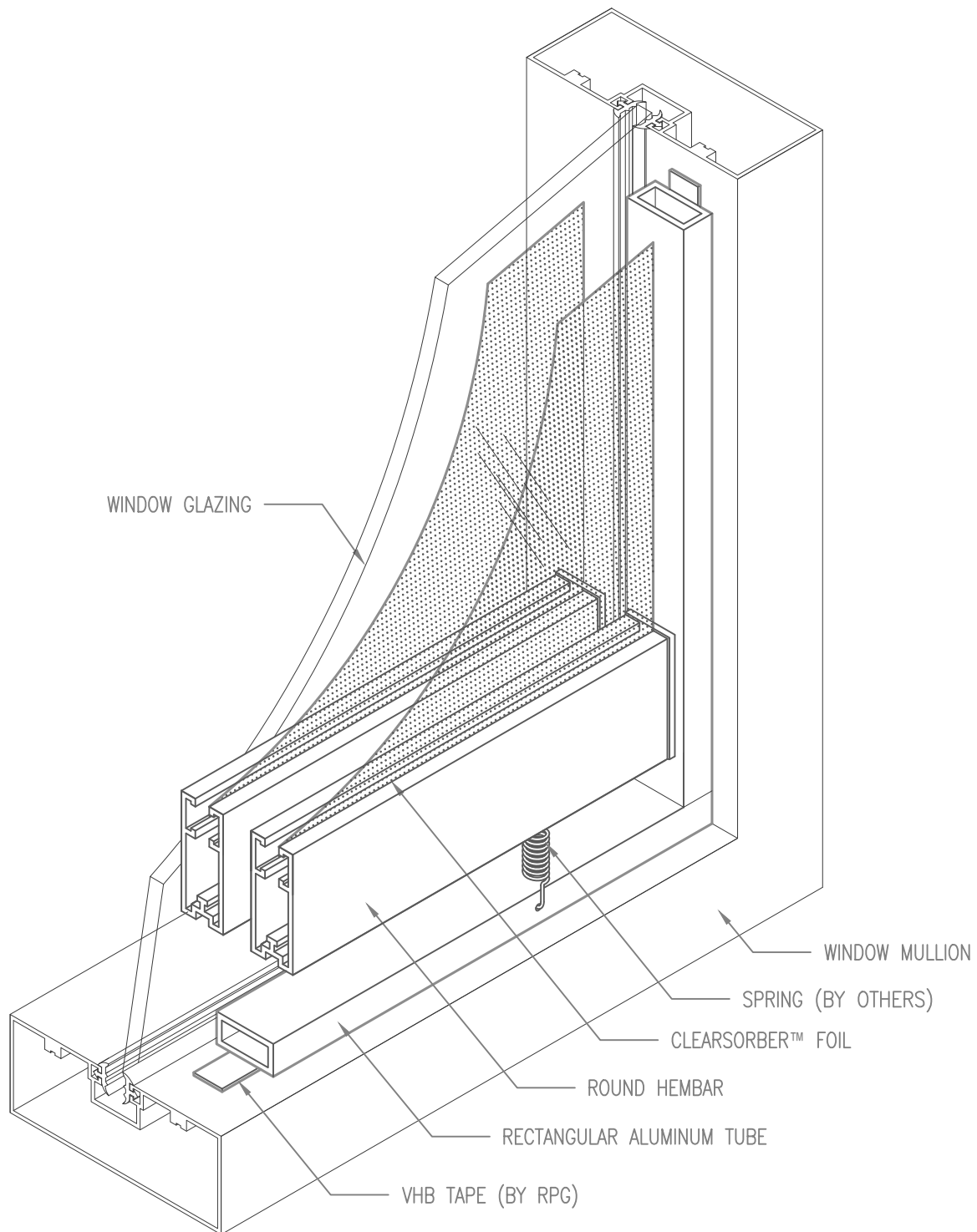
CLEARSORBER™ FOIL (DUAL LAYER) PENETRATION FREE MOUNTING TUBE/SPRING/DUAL HEMBAR MOUNTING
