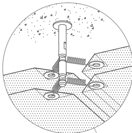
TWO CORNER PIN ATTACHMENT
