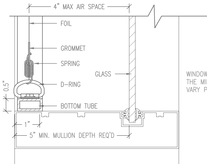
SINGLE LAYER WITH 4" TO GLASS
