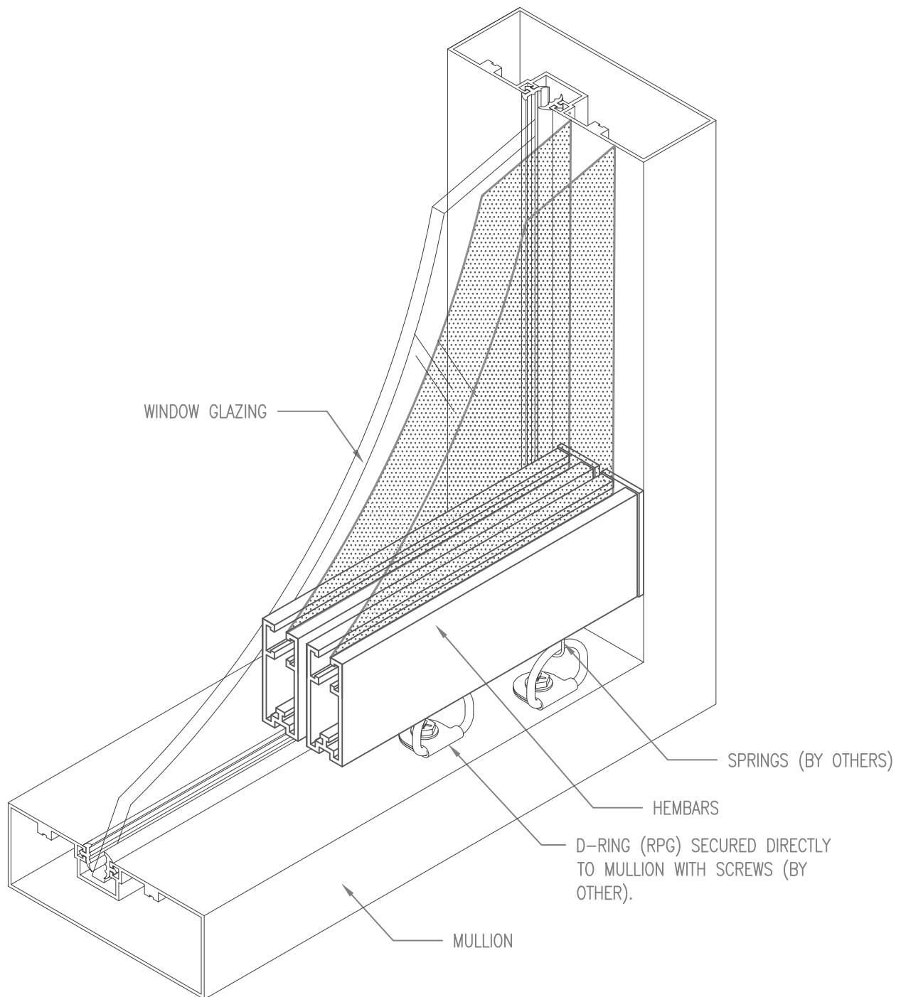
CLEARSORBER™ FOIL (DUAL LAYER) D-RING/SPRING/DUAL HEMBAR DIRECT MOUNT TO WINDOW MULLION
