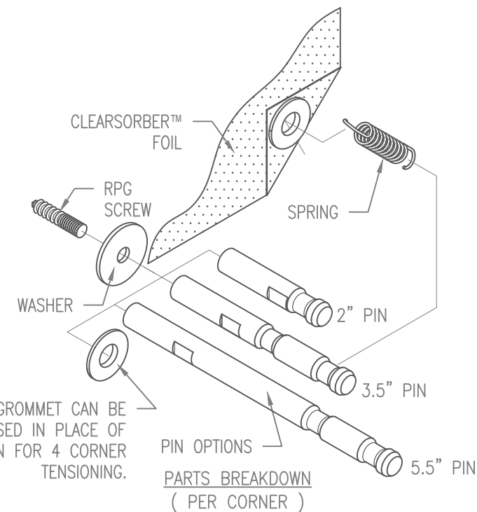
THREE CORNER PIN ATTACHMENT
