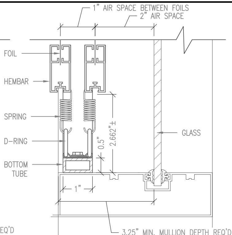
DUAL LAYER WITH 2" TO GLASS
