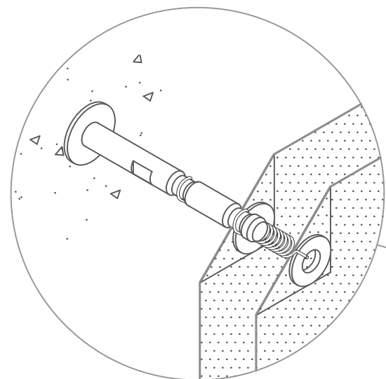
SINGLE CORNER PIN ATTACHMENT
