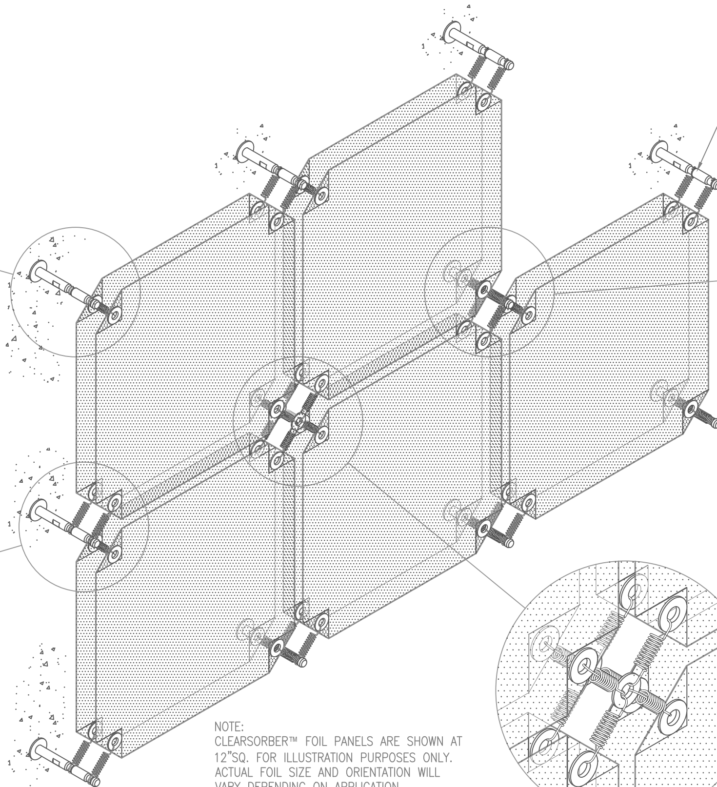
FOUR CORNER GROMMET ATTACHMENT (PIN (NOT SHOWN) CAN BE USED IN PLACE OF GROMMET)
