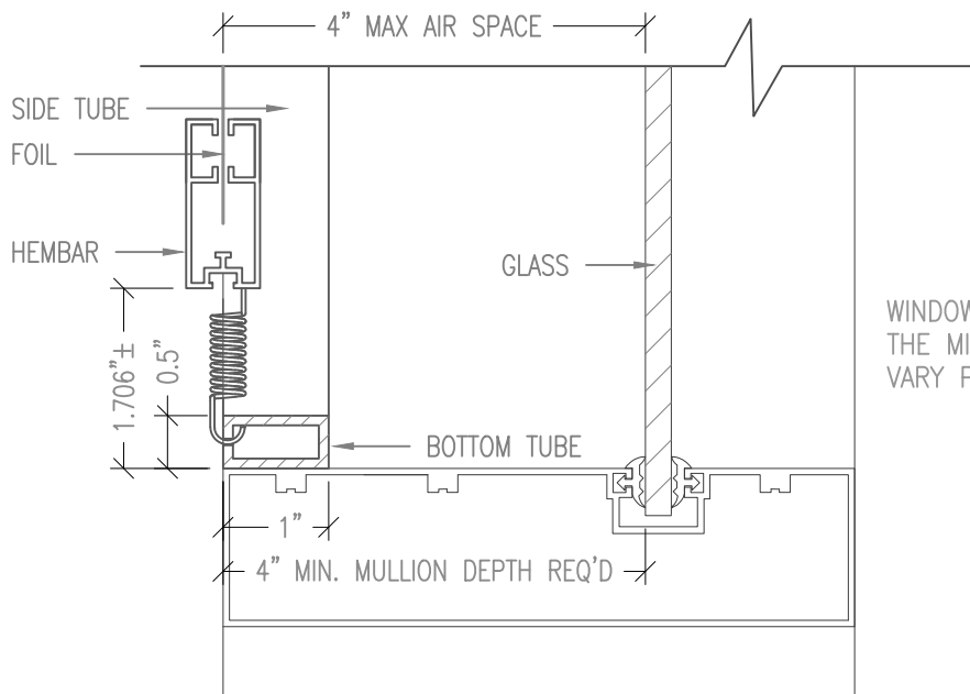
SINGLE LAYER WITH 4" TO GLASS
