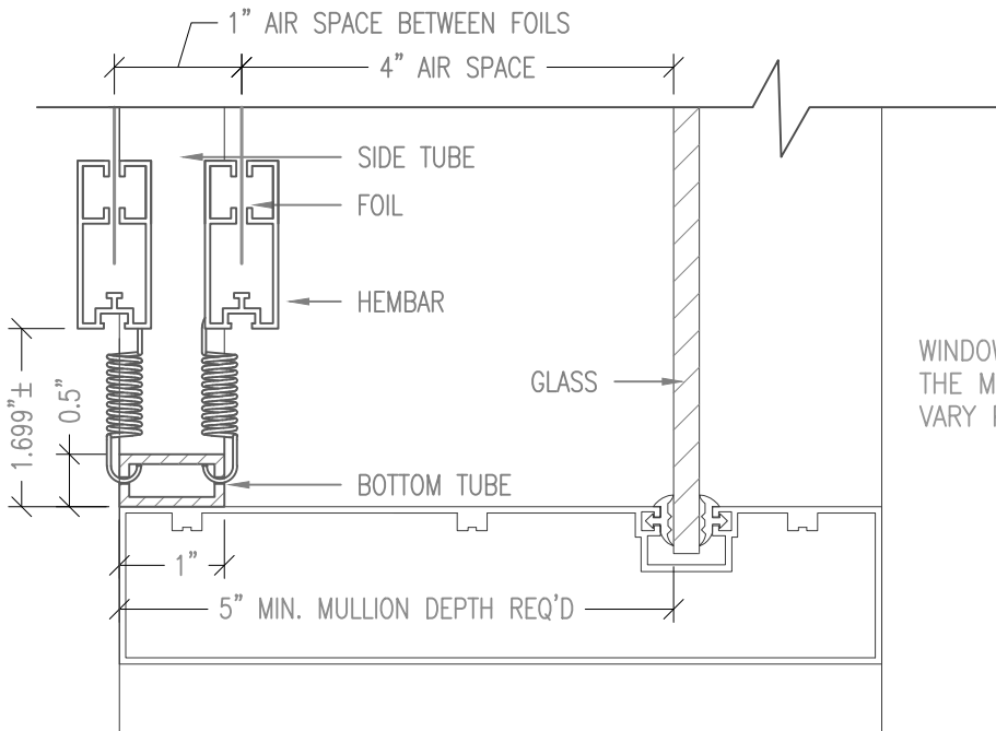
DUAL LAYER WITH 4" TO GLASS
