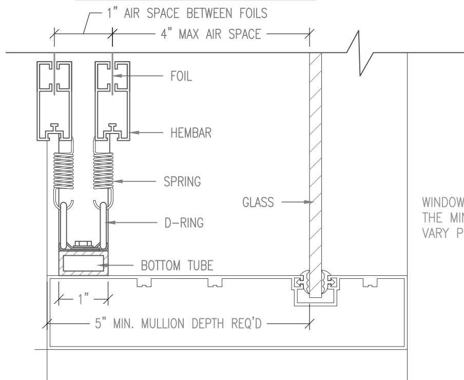
DUAL LAYER WITH 4" TO GLASS
