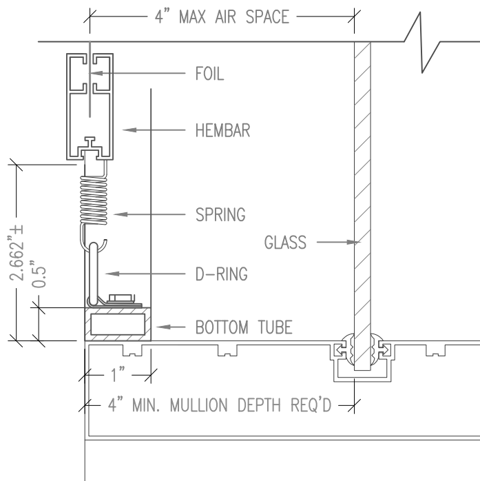
SINGLE LAYER WITH 4" TO GLASS
