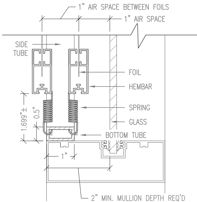
DUAL LAYER WITH 1" TO GLASS
