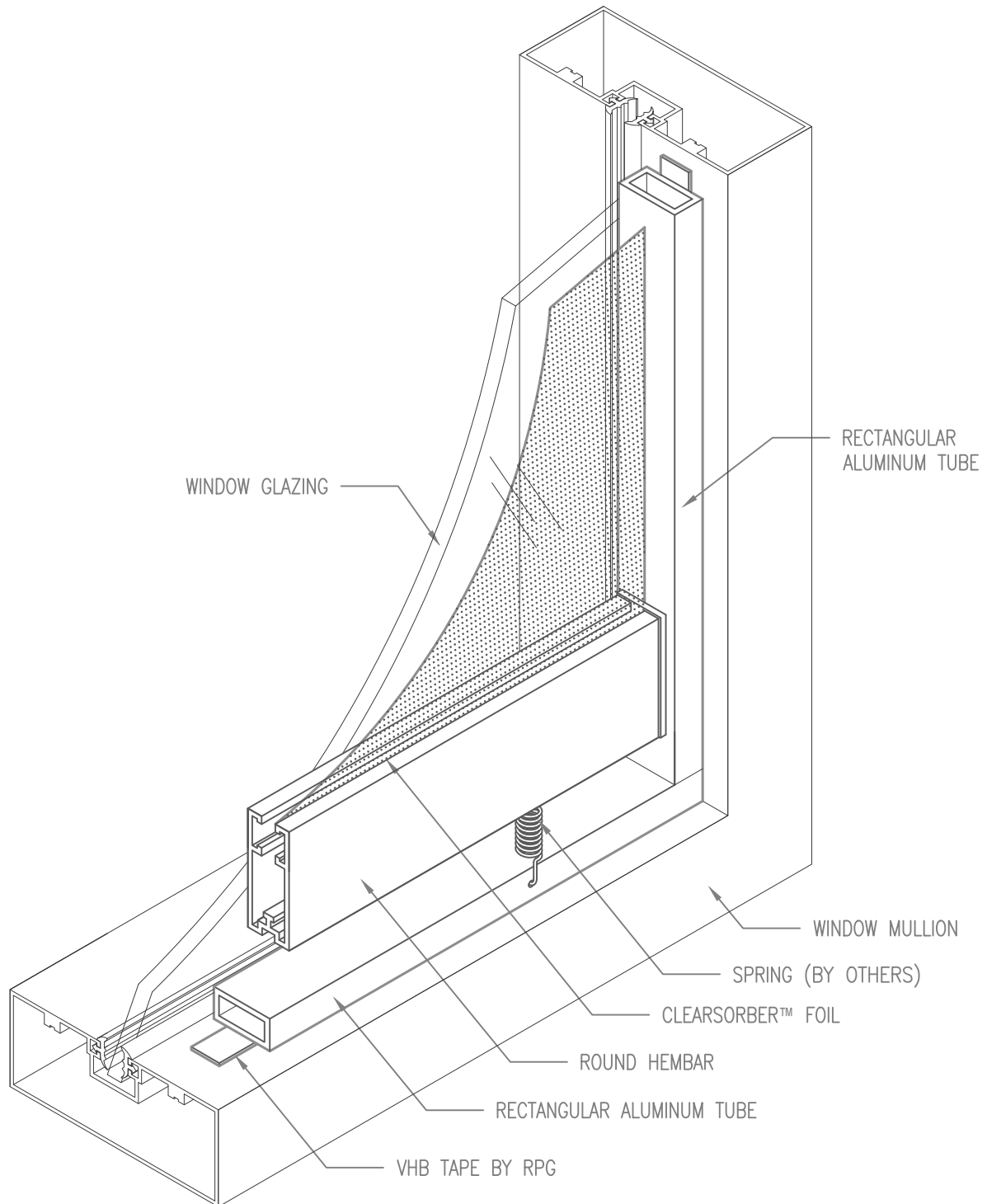
CLEARSORB™ FOIL (SINGLE LAYER) PENETRATION FREE MOUNTING TUBE/SPRING/HEMBAR MOUNTING
