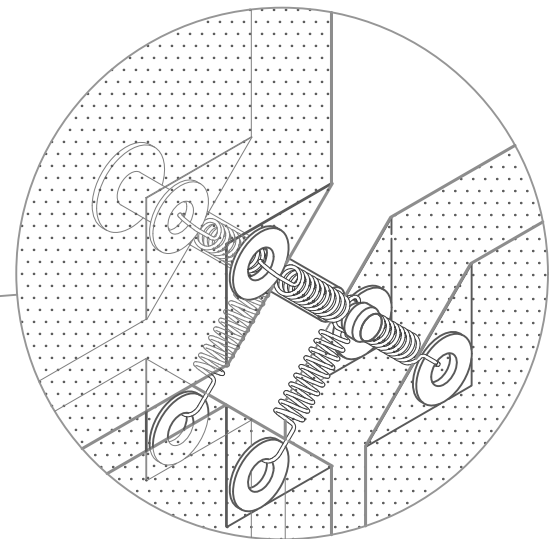
THREE CORNER PIN ATTACHMENT
