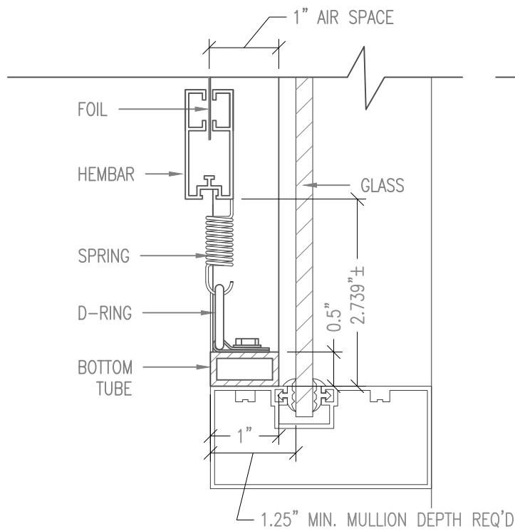
SINGLE LAYER WITH 1" TO GLASS
