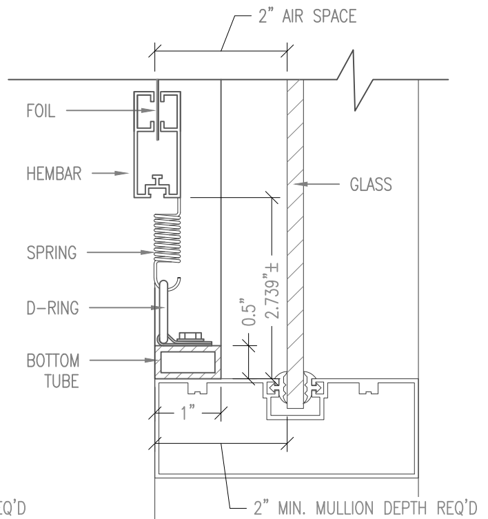
SINGLE LAYER WITH 2" TO GLASS
