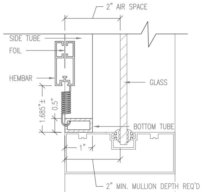
SINGLE LAYER WITH 2" TO GLASS
