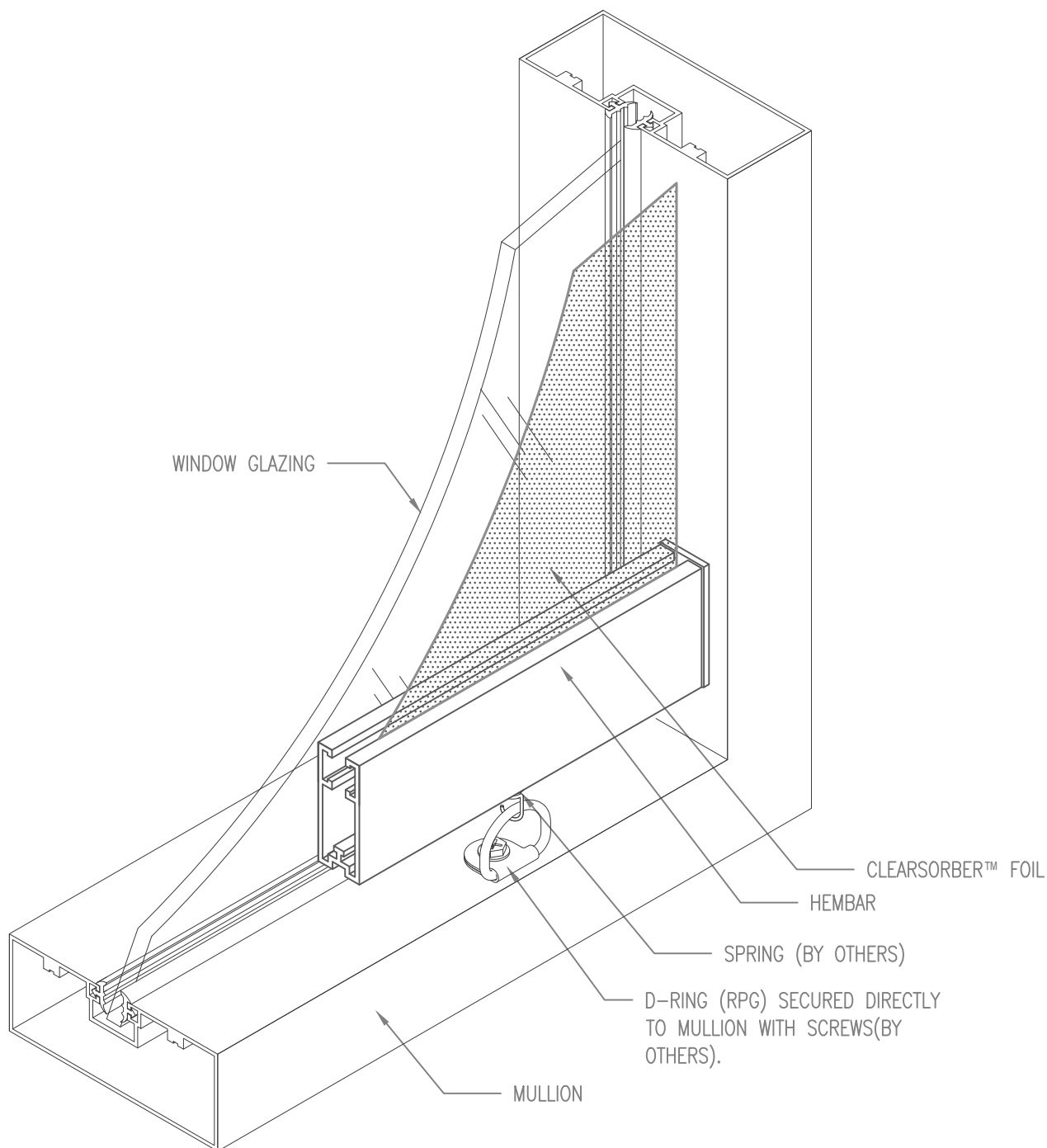
CLEARSORBER™ FOIL (SINGLE LAYER) D-RING/SPRING/HEMBAR DIRECT MOUNT TO WINDOW MULLION
