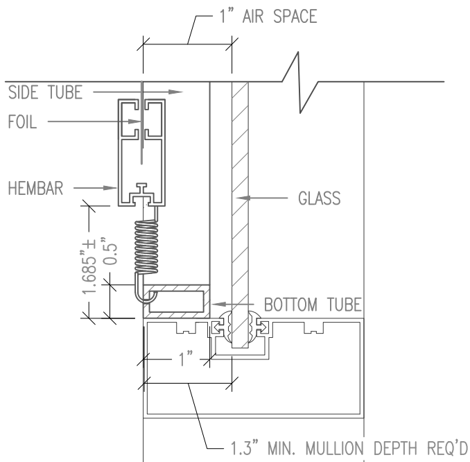
SINGLE LAYER WITH 1" TO GLASS
