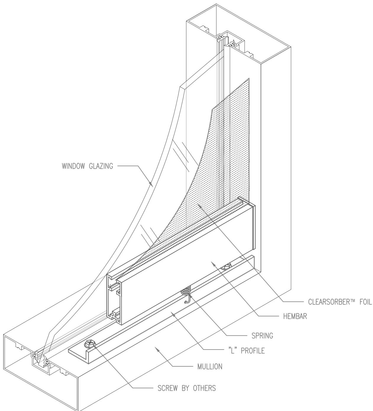
CLEARSORBER™ FOIL (SINGLE LAYER) DIRECT MOUNT TO WINDOW MULLION "L"-PROFILE/SPRING/HEMBAR
