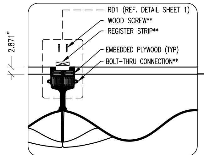
JOINING DETAIL (SECTION)
