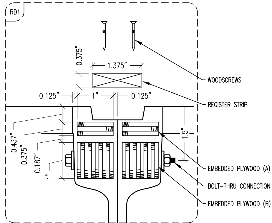
MOUNTING DETAIL – JOINING
