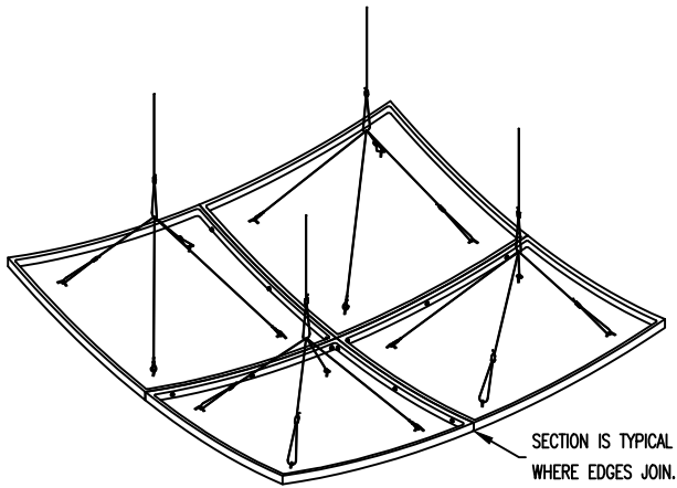
BIRADIAL ARRAY JOINED & SUSPENDED
