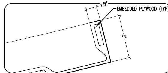
END DETAIL (SECTION)
