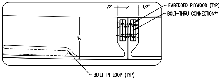
JOINING DETAIL (SECTION)
