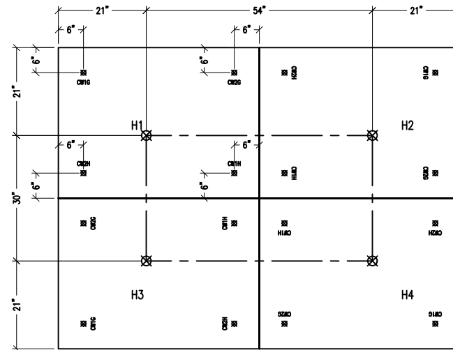
TOP VIEW W/ CROSS WIRE & HANG POINTS
