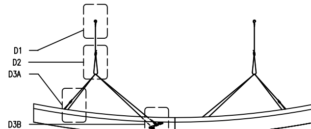
FRONT VIEW OF BIRADIALS 3 & 4
