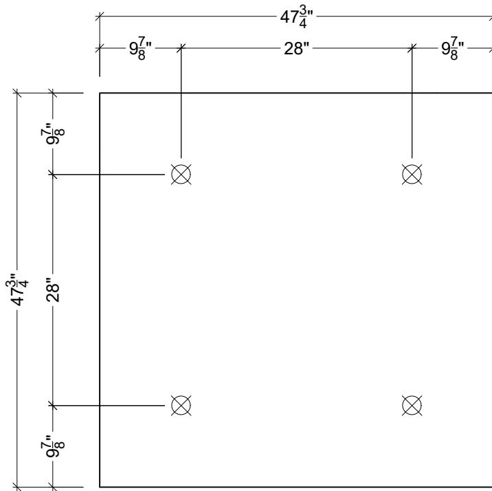
TOP VIEW W/ HANG POINTS
