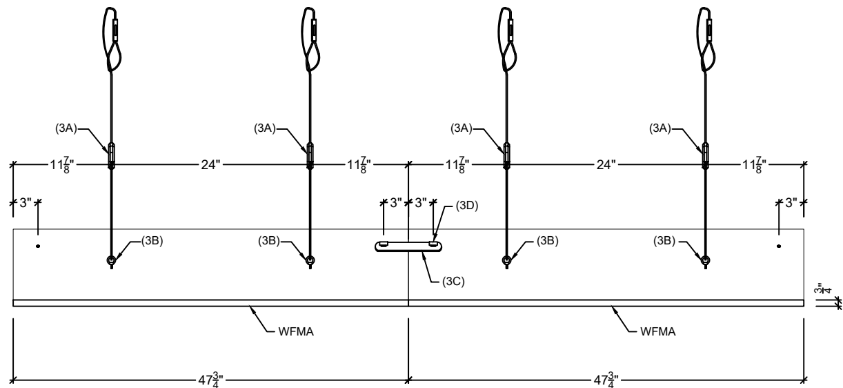
2 PLAN SECTION SCALE: 3/4"=1'-0" ARCH'T REF.:
