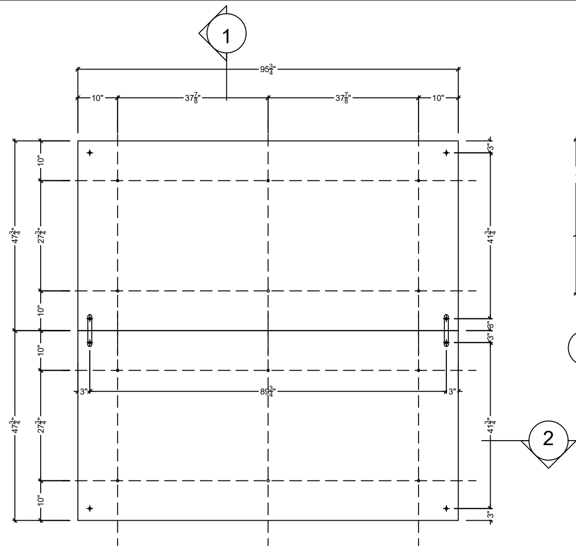
1 ELEVATION SCALE: 3/4"=1'-0" ARCH'T REF.:
