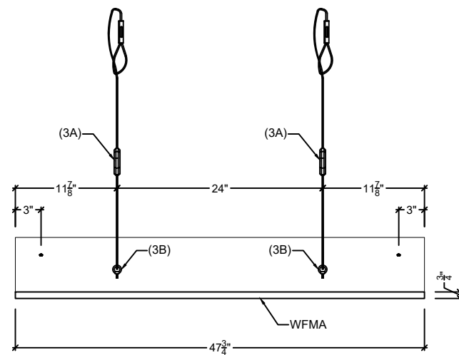
I PLAN SECTION SCALE: 1"=1'-0" ARCH'T REF.:
